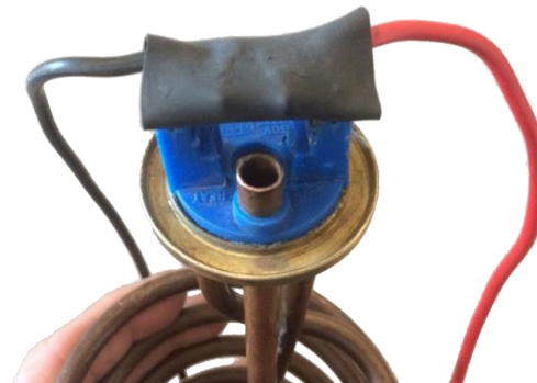
Figure 4.6 Element connector fitted to flange-type element
