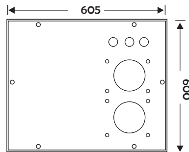
GLAND PLATE 2 FANS (VENTED) Code: FANTRAY02.IP55-ALZ
