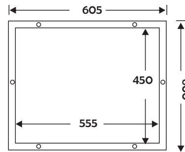
BOTTOM ENTRY
