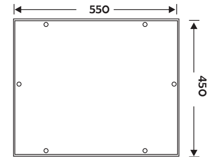
GLAND PLATE PLAIN
