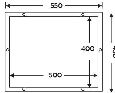
BOTTOM ENTRY
