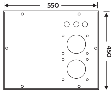
GLAND PLATE 2 FANS (VENTED)
