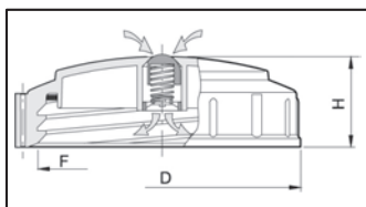
Lid with spring breather and gasket
