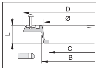
Threaded ring for flat surfaces
