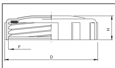
Transparent closed lid complete with gasket
