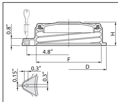
Closed lid "DOT" with gasket
