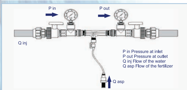
Typical Installation
