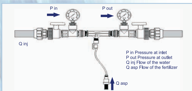
Typical Installation
