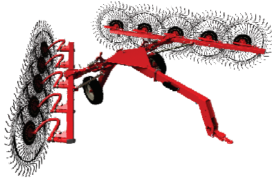
MASTER RAKE | Carted V-Rake
